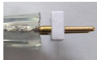
Side view after securing of the 4-pin connector
